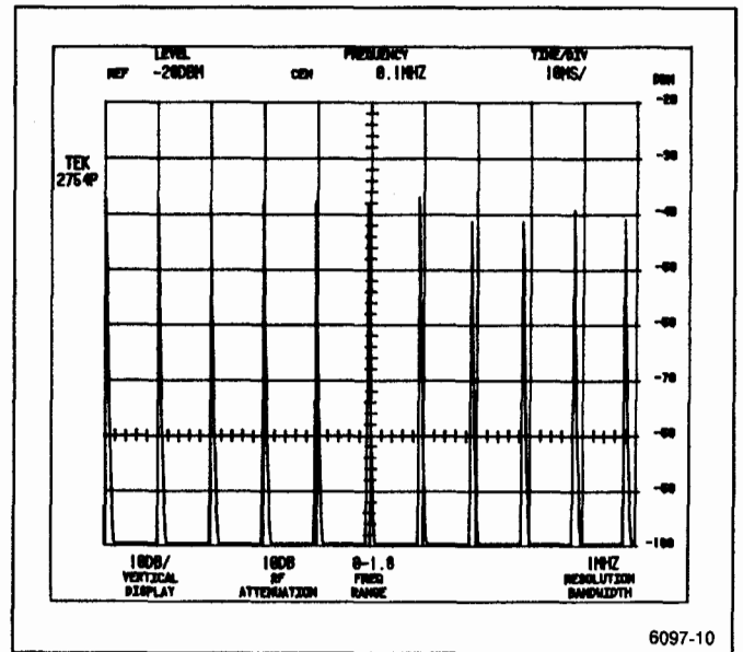
Figure 4-7. Typical display for measuring Time/Div accuracy.
