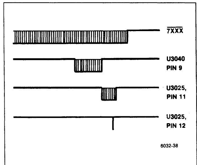
Figure 6-29. RAM select output in relation to OXXX.
