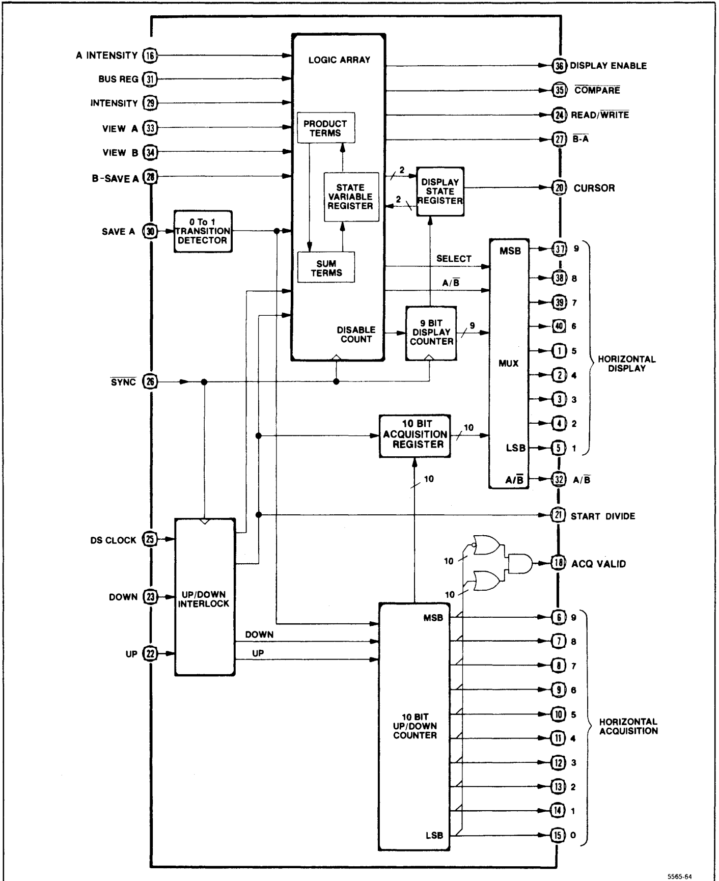
Figure 7-16. Horizontal control IC block diagram.
